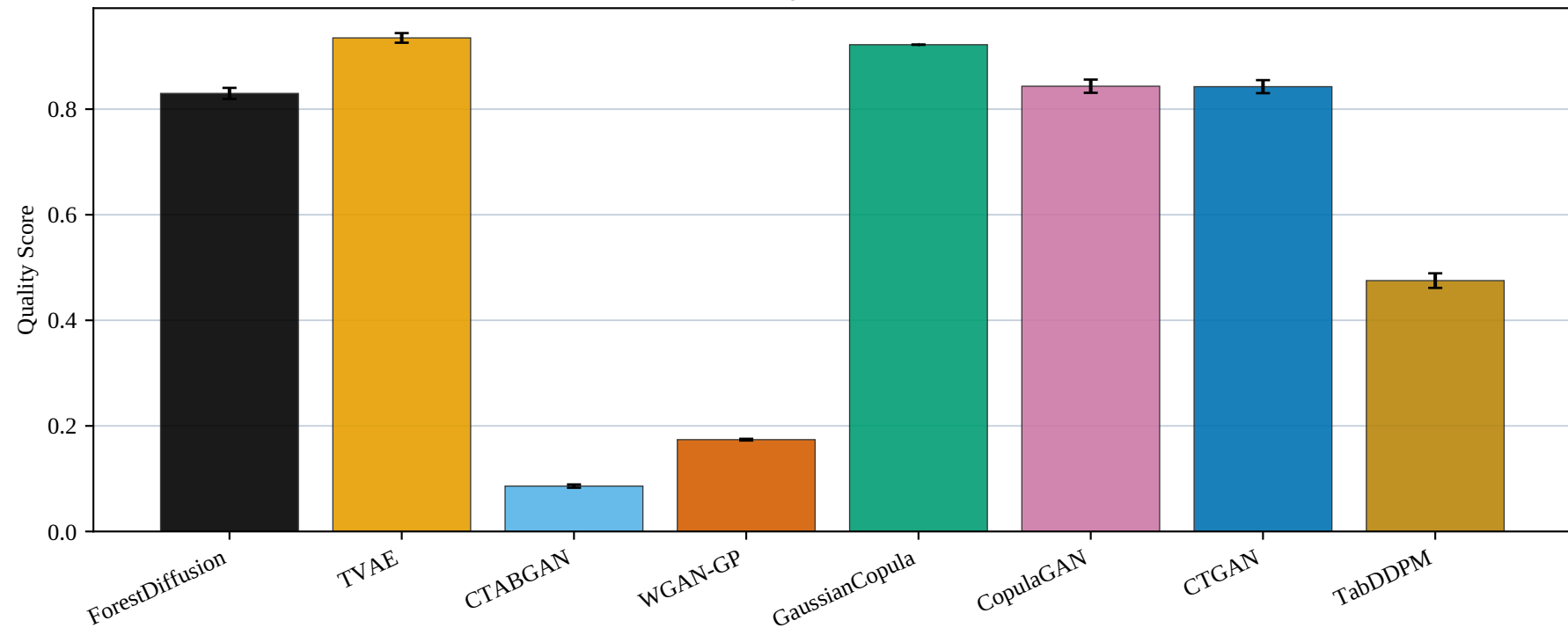
Forest Cover — Quality Score (mean \pm SD, 10 seeds)
